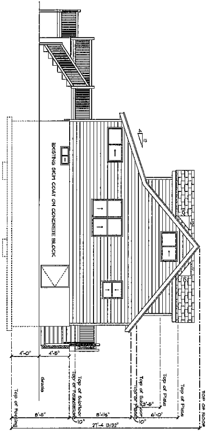
EXISTING LEFT ELEVATION
