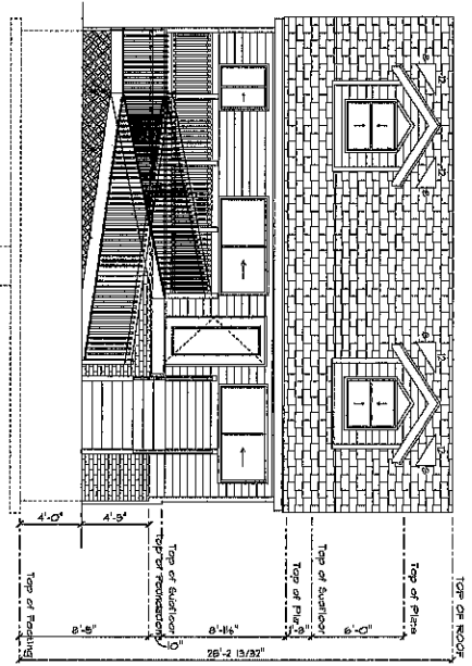
EXISTING REAR (LAKE) ELEVATION
