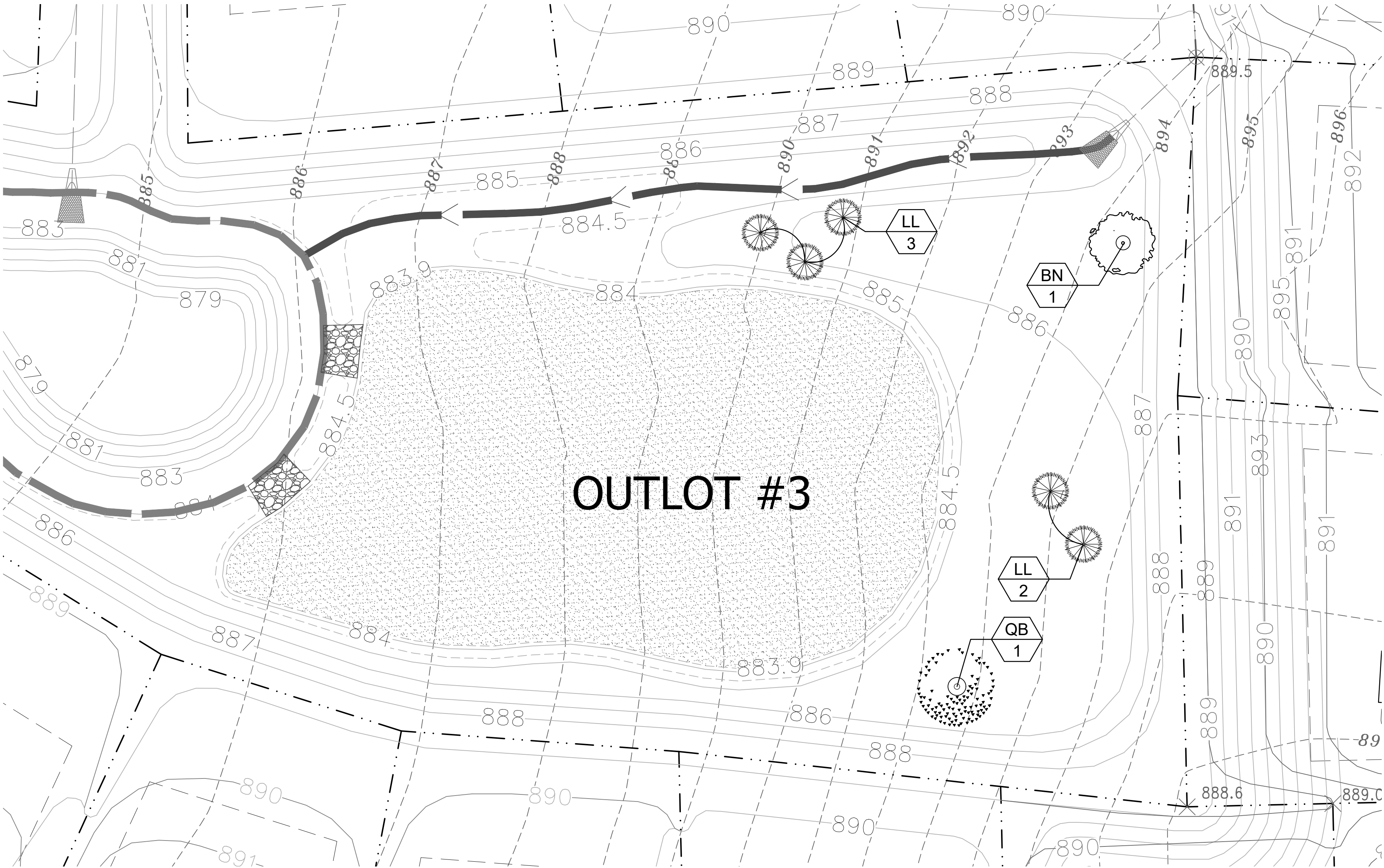
OUTLOT #3 LAYOUT
