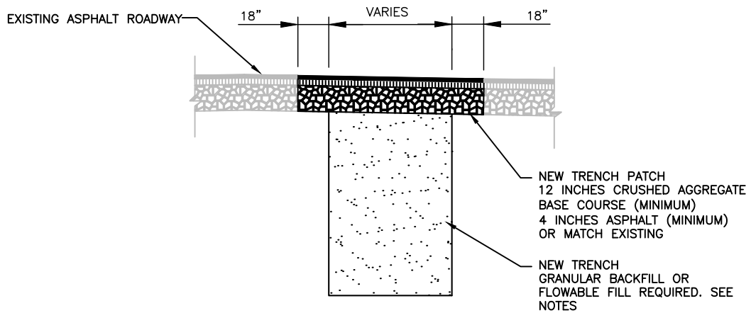
ASPHALT ROADWAY TRENCH PATCH CROSS SECTION
