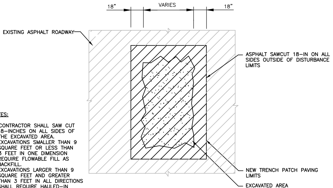
ASPHALT ROADWAY TRENCH PATCH PLAN VIEW
