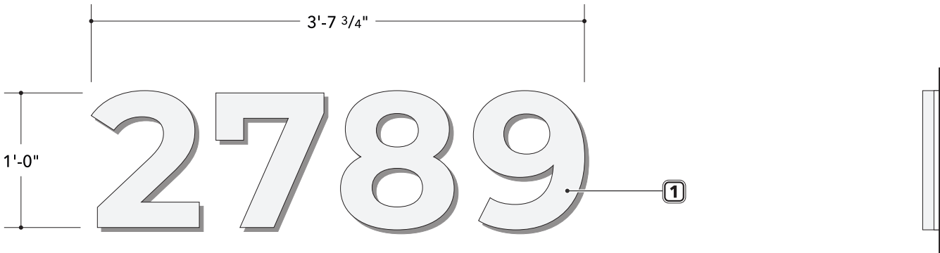
3 Sign Detail
