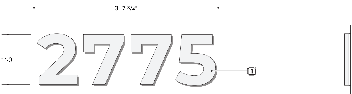
3 Sign Detail
