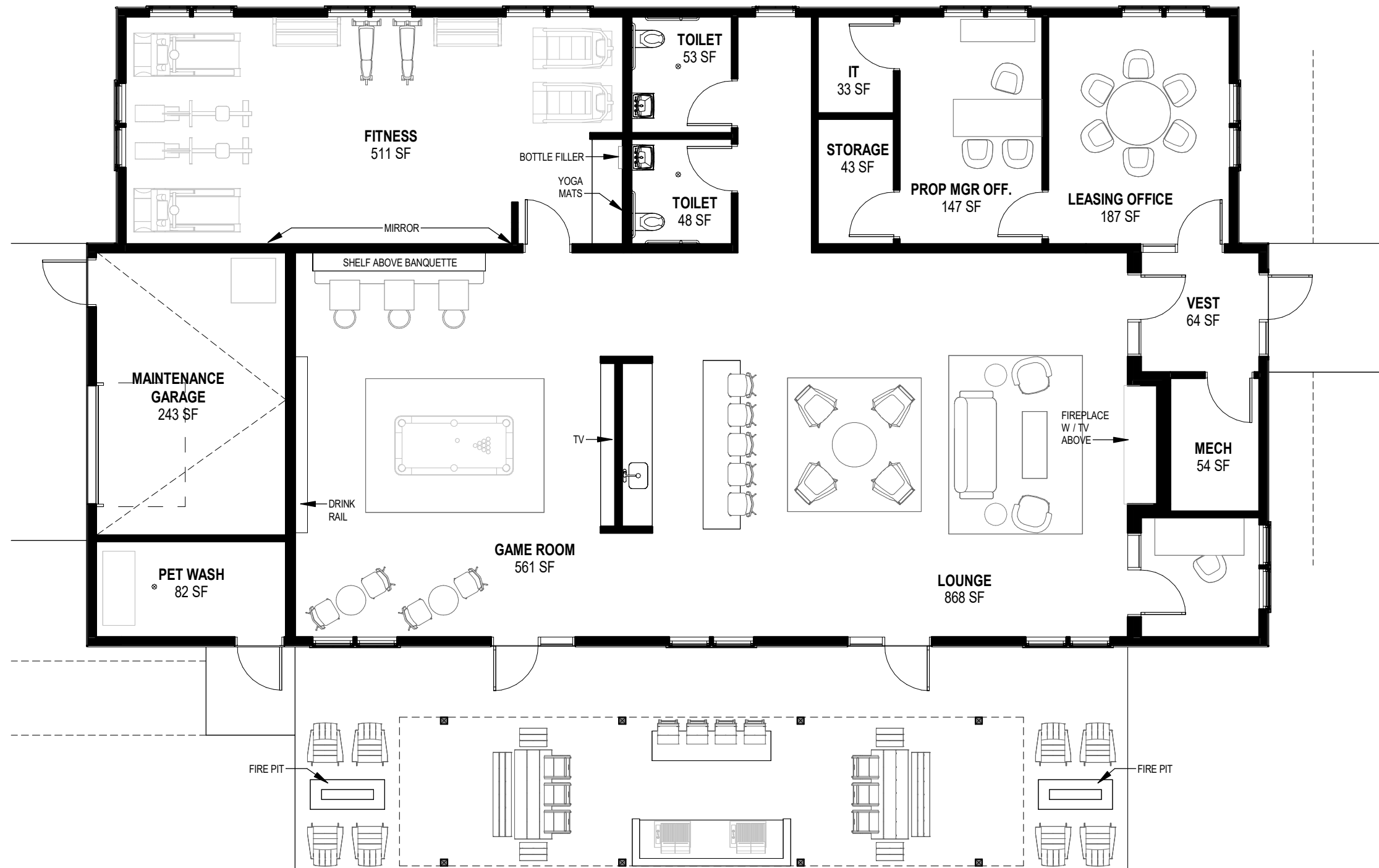
1 FLOOR PLAN 1/8" = 1'-0"
